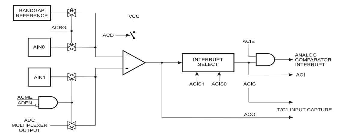
Figure 20-1. Analog Comparator Block Diagram (1)(2)
