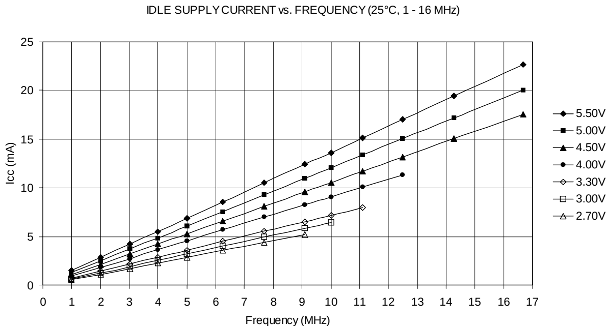
Figure 28-7. Idle Supply Current vs. Frequency (1 - 16 MHz)
