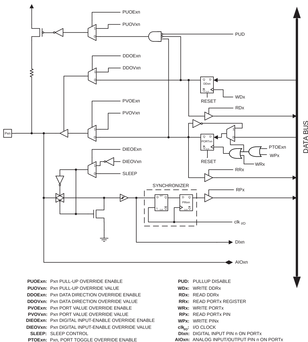
Figure 9-5. Alternate Port Functions (1)
