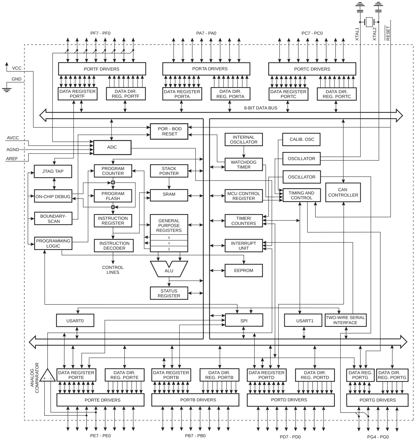
Figure 1-1. Block Diagram
