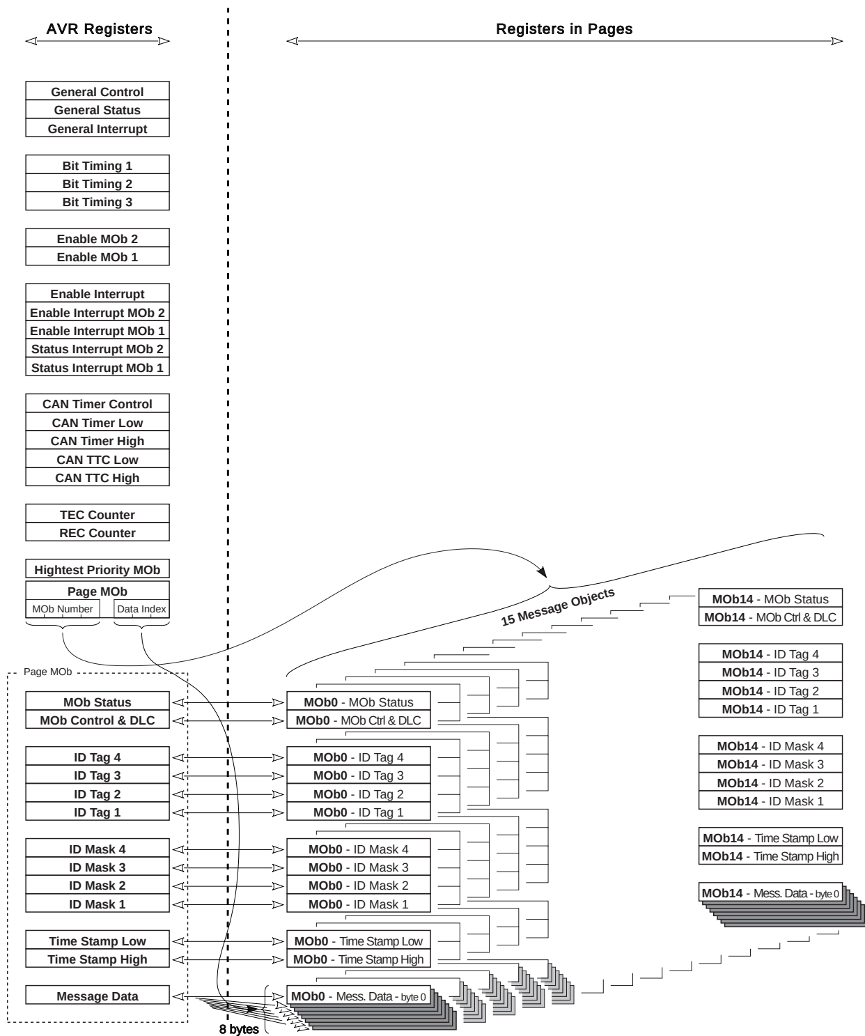
Figure 19-15. Registers Organization
