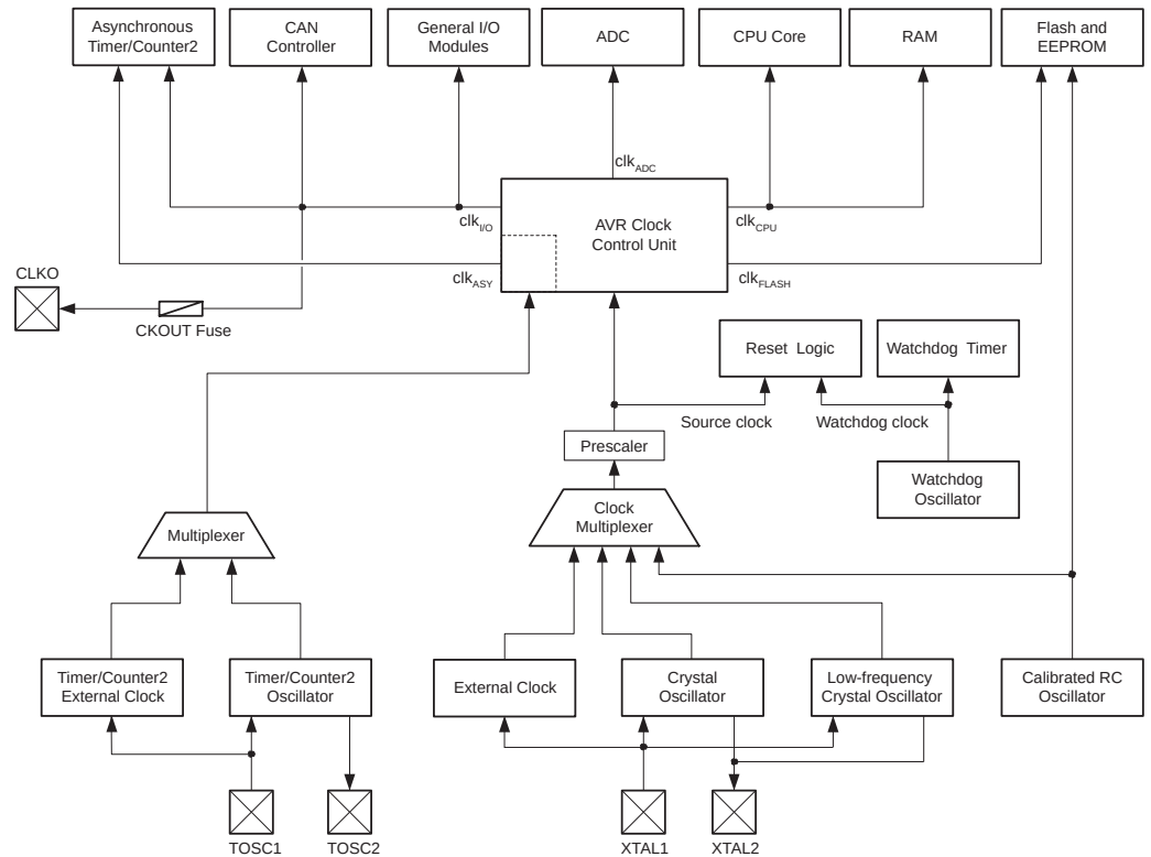
Figure 5-1. Clock Distribution
