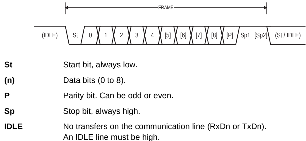
Figure 17-4. Frame Formats
