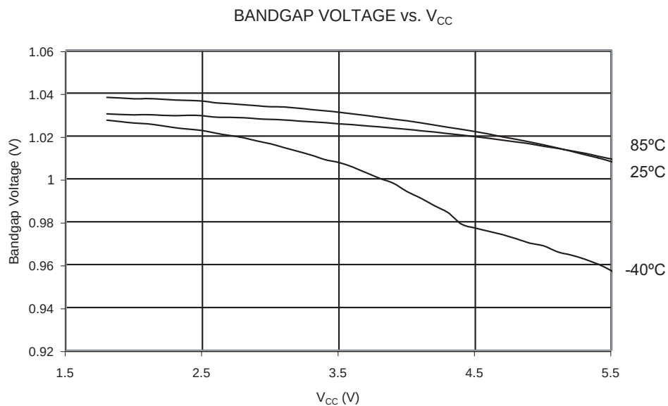
Figure 111. Bandgap Voltage vs. V_{CC}
