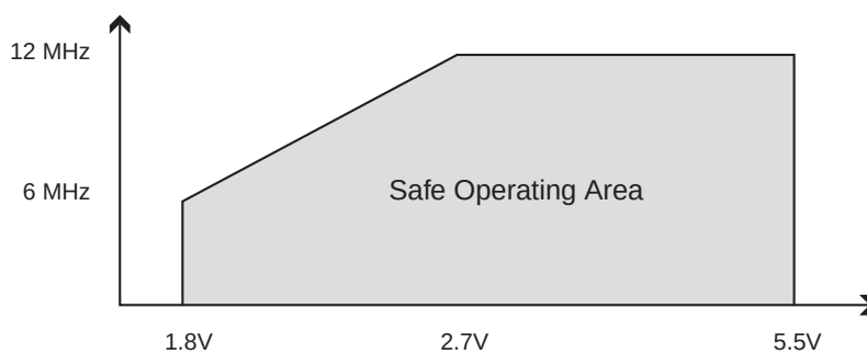
Figure 61. Maximum Frequency vs. V_{CC} , ATtiny13V
