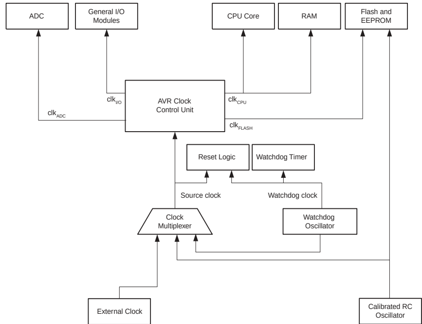
Figure 11. Clock Distribution
