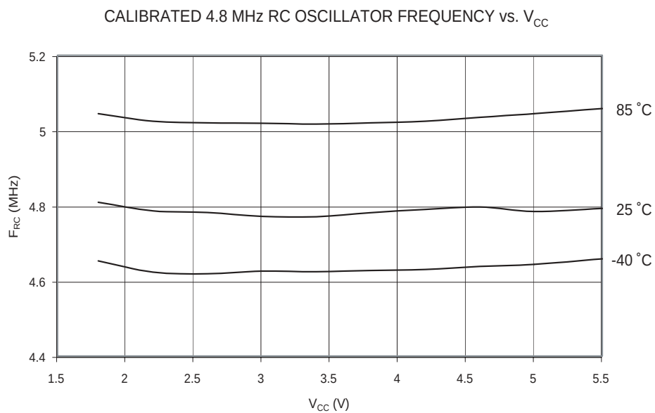
Figure 118. Calibrated 4.8 MHz RC Oscillator Frequency vs. V_{CC}
