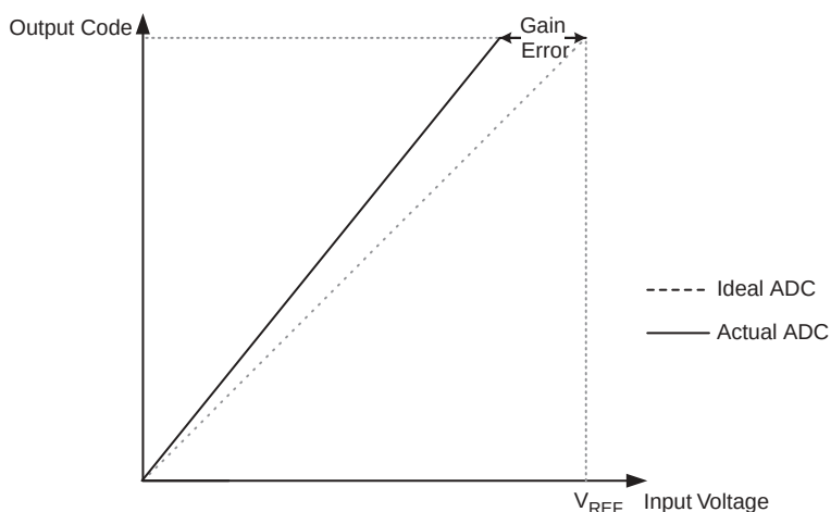
Figure 48. Gain Error
