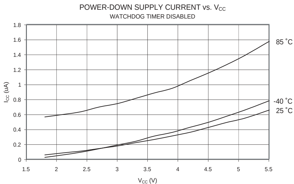
Figure 75. Power-Down Supply Current vs. V_{CC} (Watchdog Timer Disabled)
