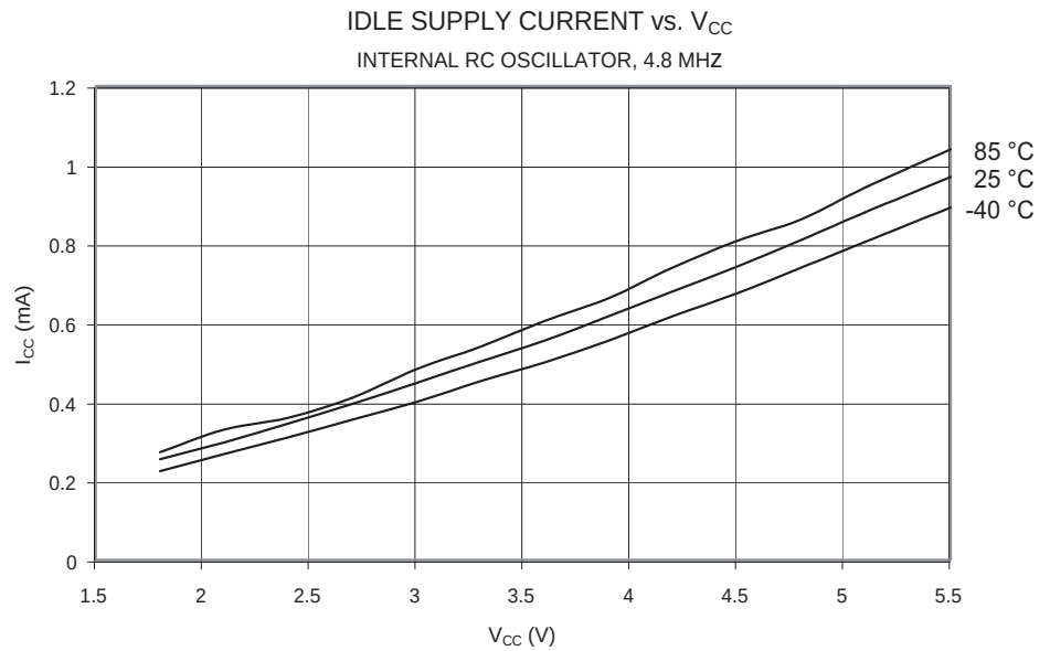
Figure 72. Idle Supply Current vs. V_{CC} (Internal RC Oscillator, 4.8 MHz)
