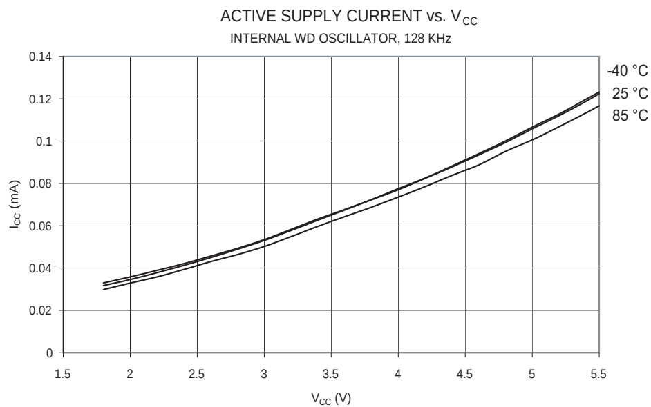
Figure 67. Active Supply Current vs. V_{CC} (Internal WDT Oscillator, 128 kHz)
