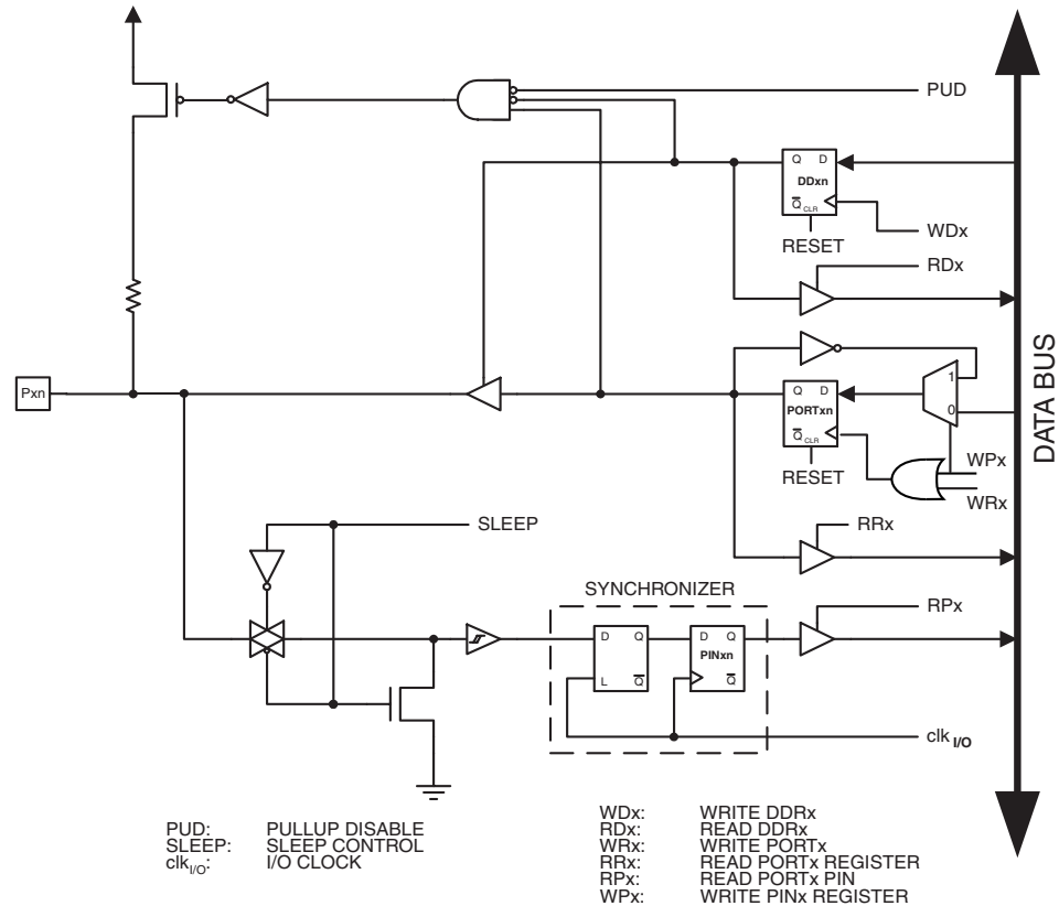
Figure 12-2. General Low Voltage Digital I/O (1)
