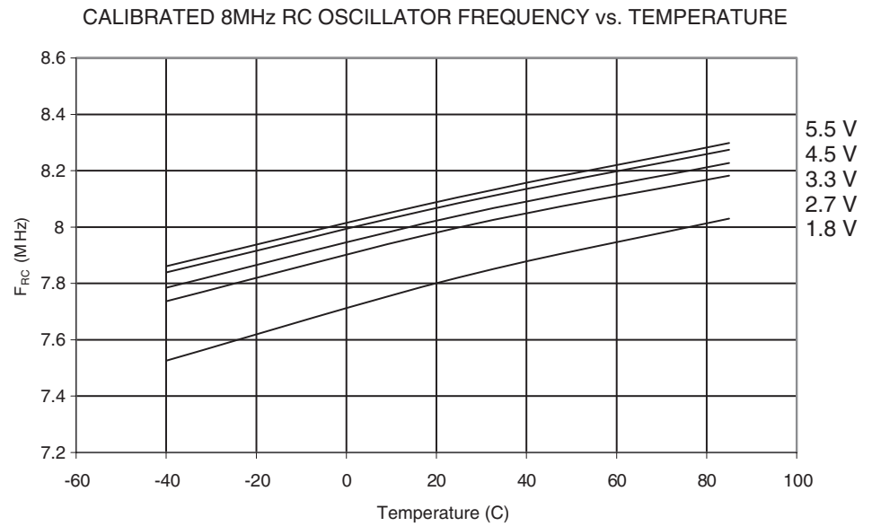
Figure 185. Calibrated 8 MHz RC Oscillator Frequency vs. Temperature
