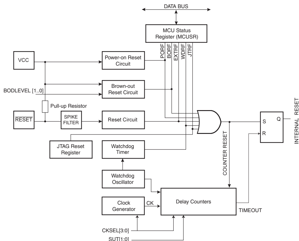
Figure 15. Reset Logic
