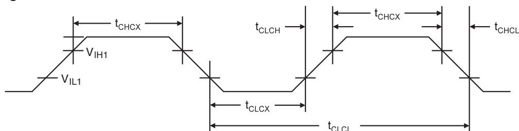
Figure 135. External Clock Drive Waveforms
