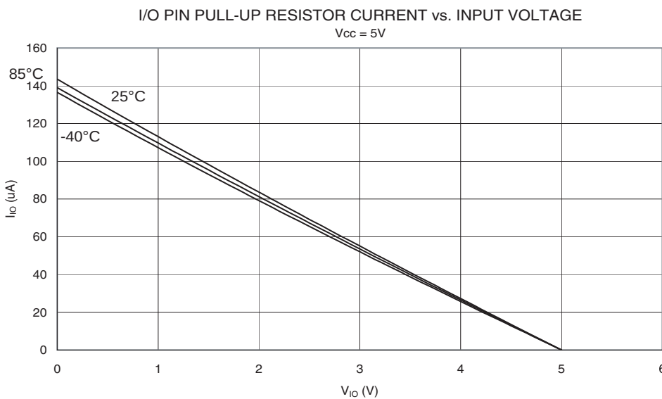
Figure 154. I/O Pin Pull-up Resistor Current vs. Input Voltage (V CC = 5V)
