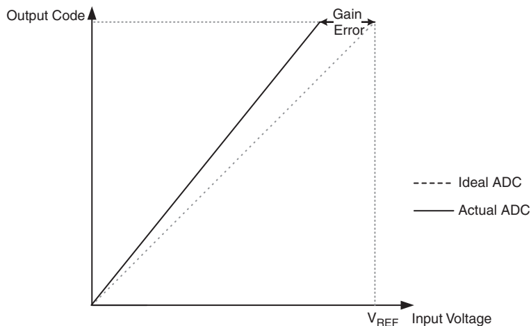
Figure 93. Gain Error
