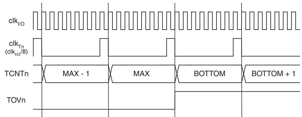
Figure 61. Timer/Counter Timing Diagram, with Prescaler ( f_{\text{clk\_I/O}}/8 )
