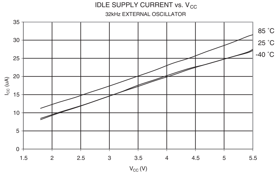
Figure 149. Idle Supply Current vs. V_{CC} (32 kHz External Oscillator)
