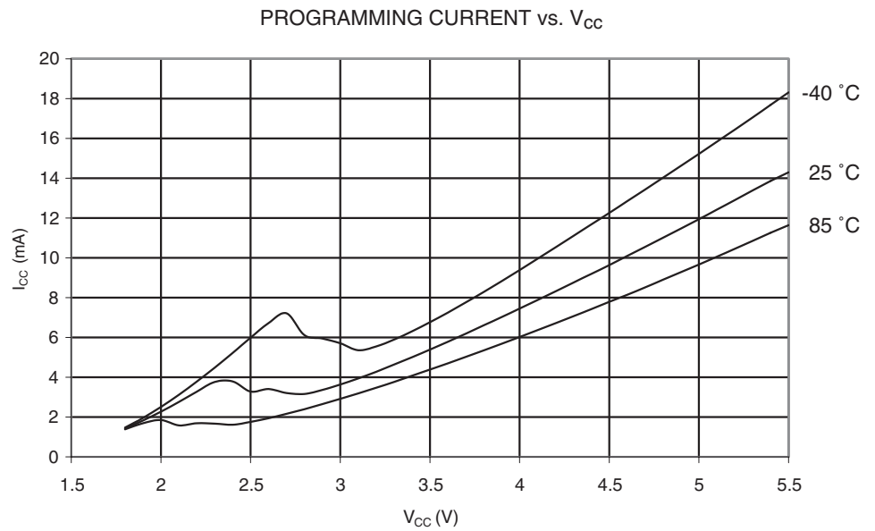
Figure 194. Programming Current vs. V_{CC}
