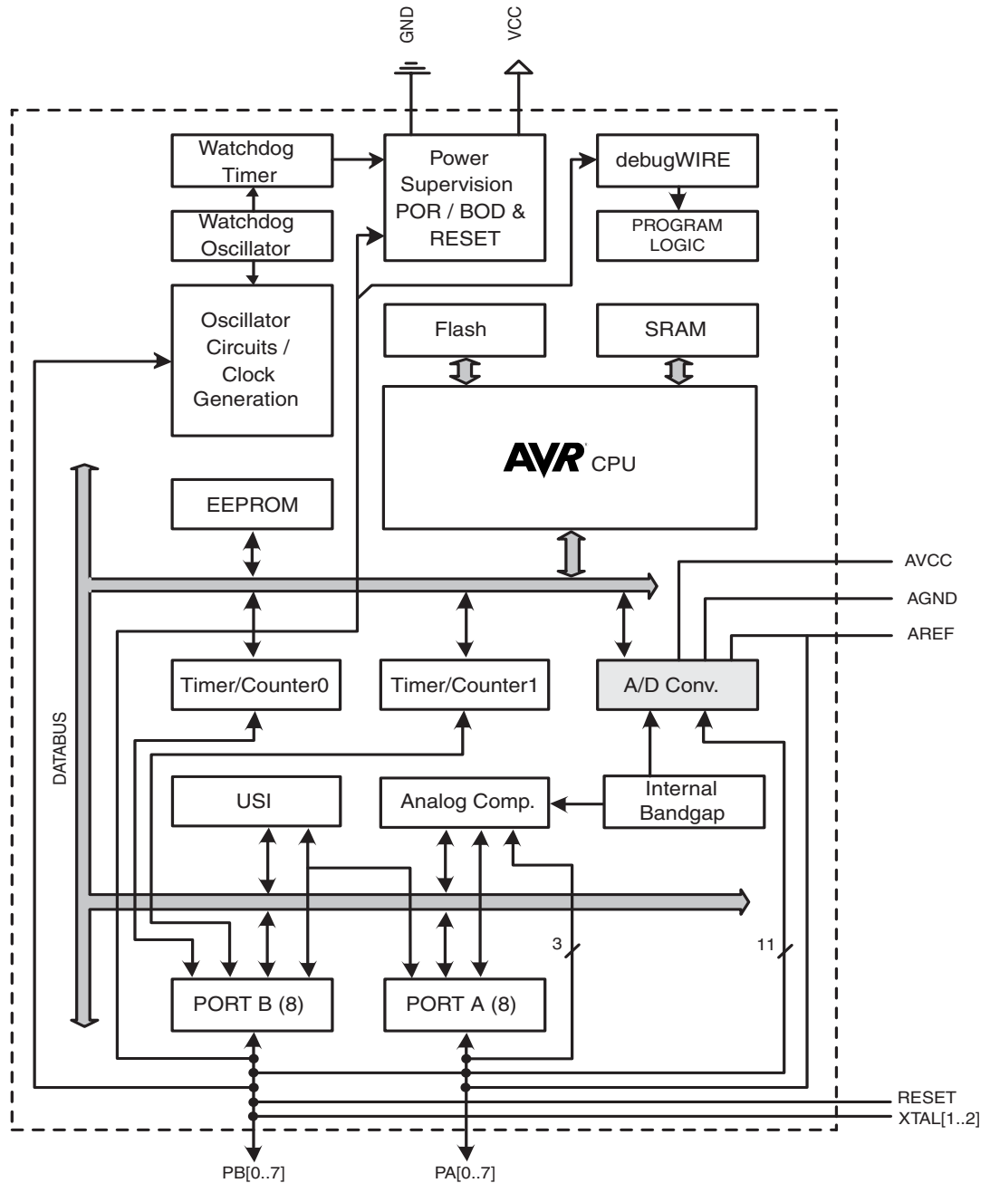
Figure 2-1. Block Diagram
