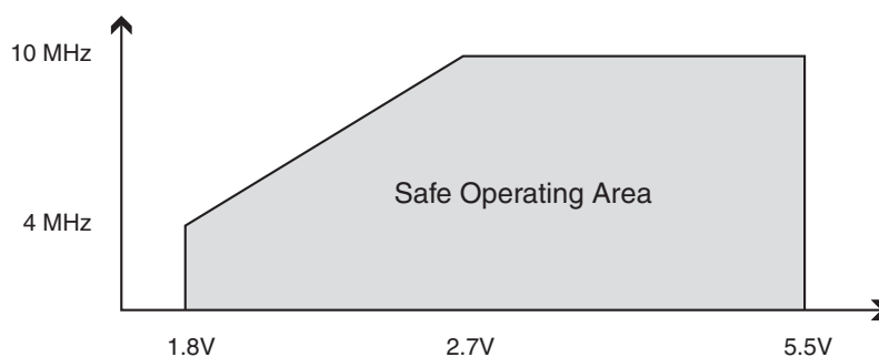
Figure 27-1. Maximum Frequency vs. V_{CC} , ATmega48V/88V/168V
