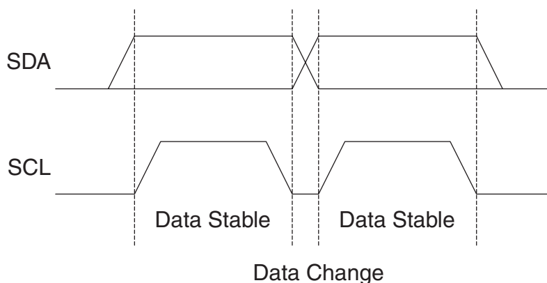
Figure 20-2. Data Validity
