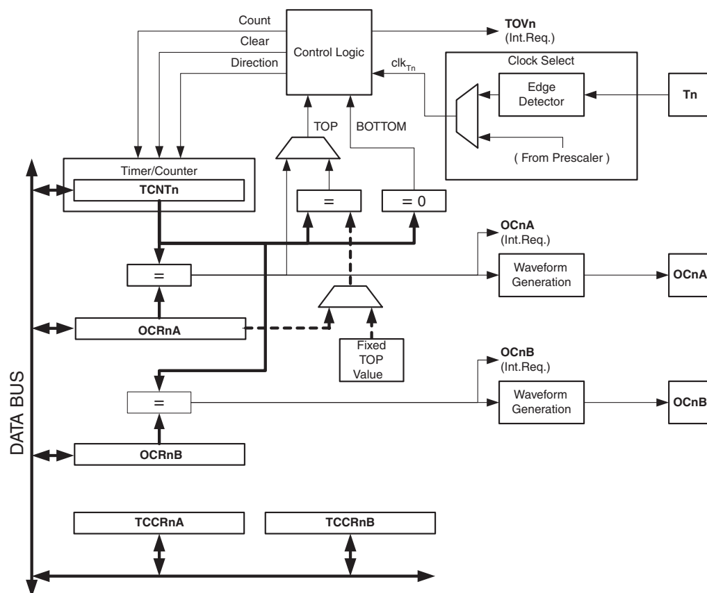
Figure 13-1. 8-bit Timer/Counter Block Diagram
