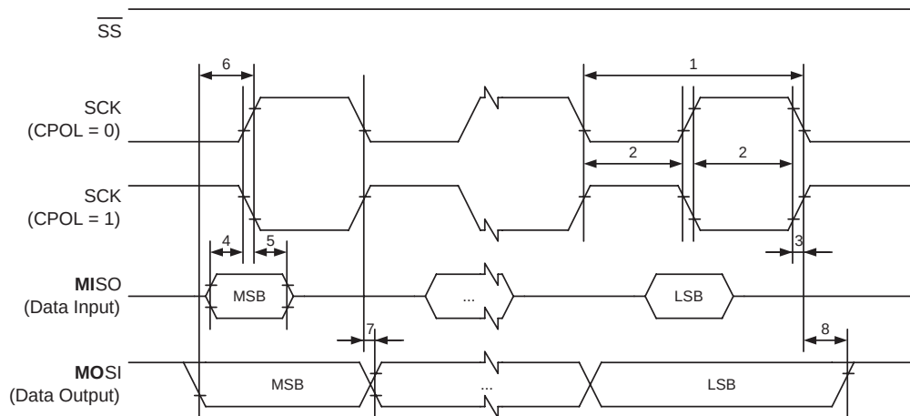
Figure 27-5. SPI Interface Timing Requirements (Master Mode)
