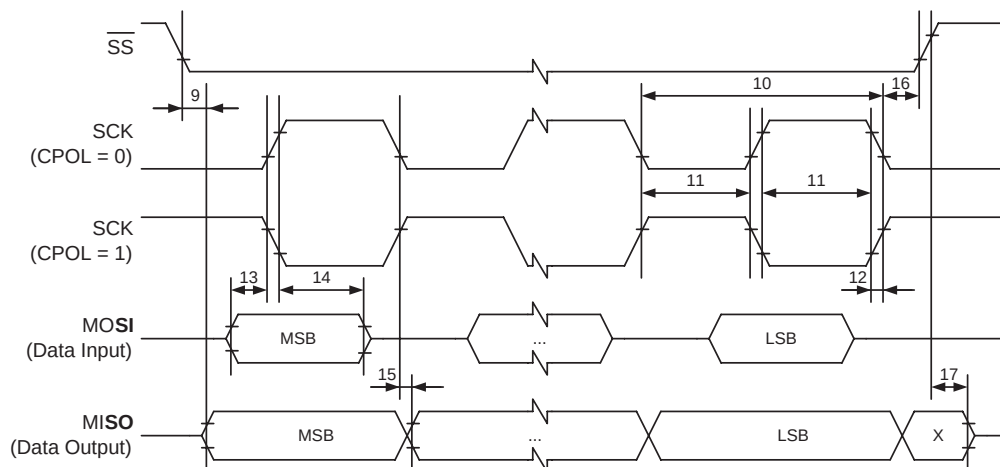
Figure 27-6. SPI Interface Timing Requirements (Slave Mode)
