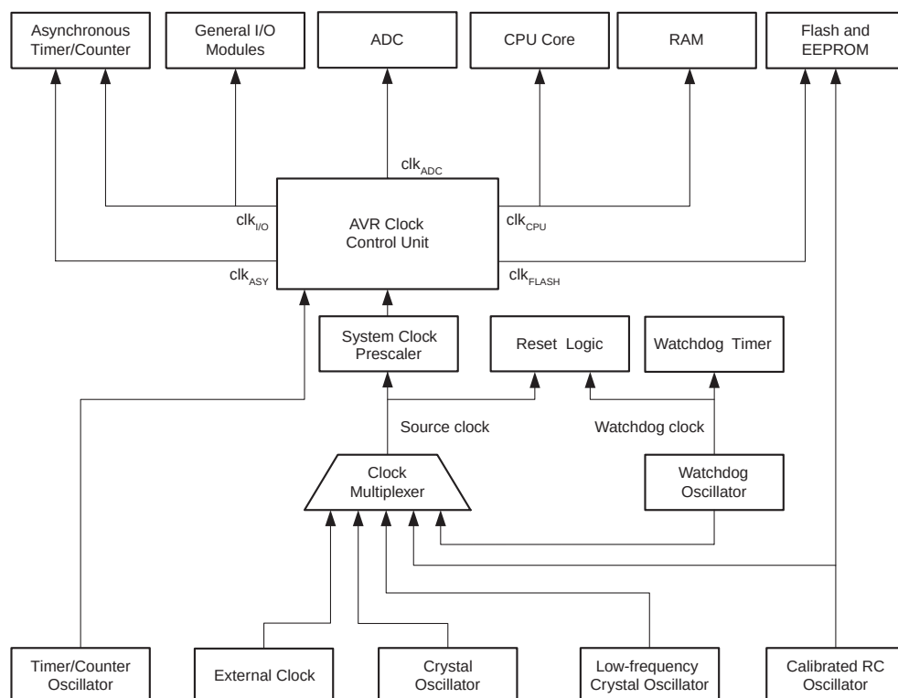
Figure 7-1. Clock Distribution
