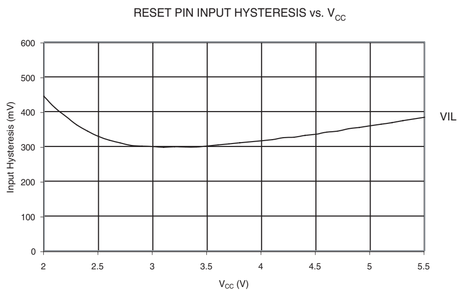
Figure 28-32. Reset Input Pin Hysteresis vs. V_{CC}
