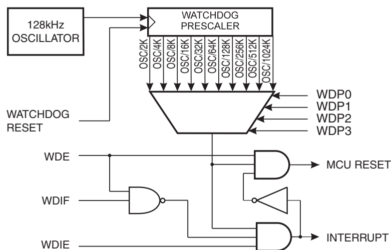
Figure 9-7. Watchdog Timer
