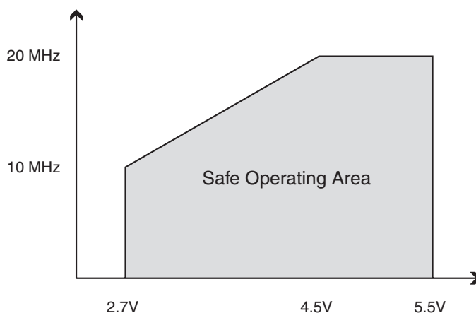
Figure 27-2. Maximum Frequency vs. V_{CC} , ATmega48/88/168
