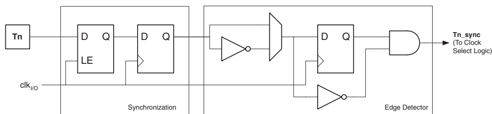
Figure 15-1. T1/T0 Pin Sampling
