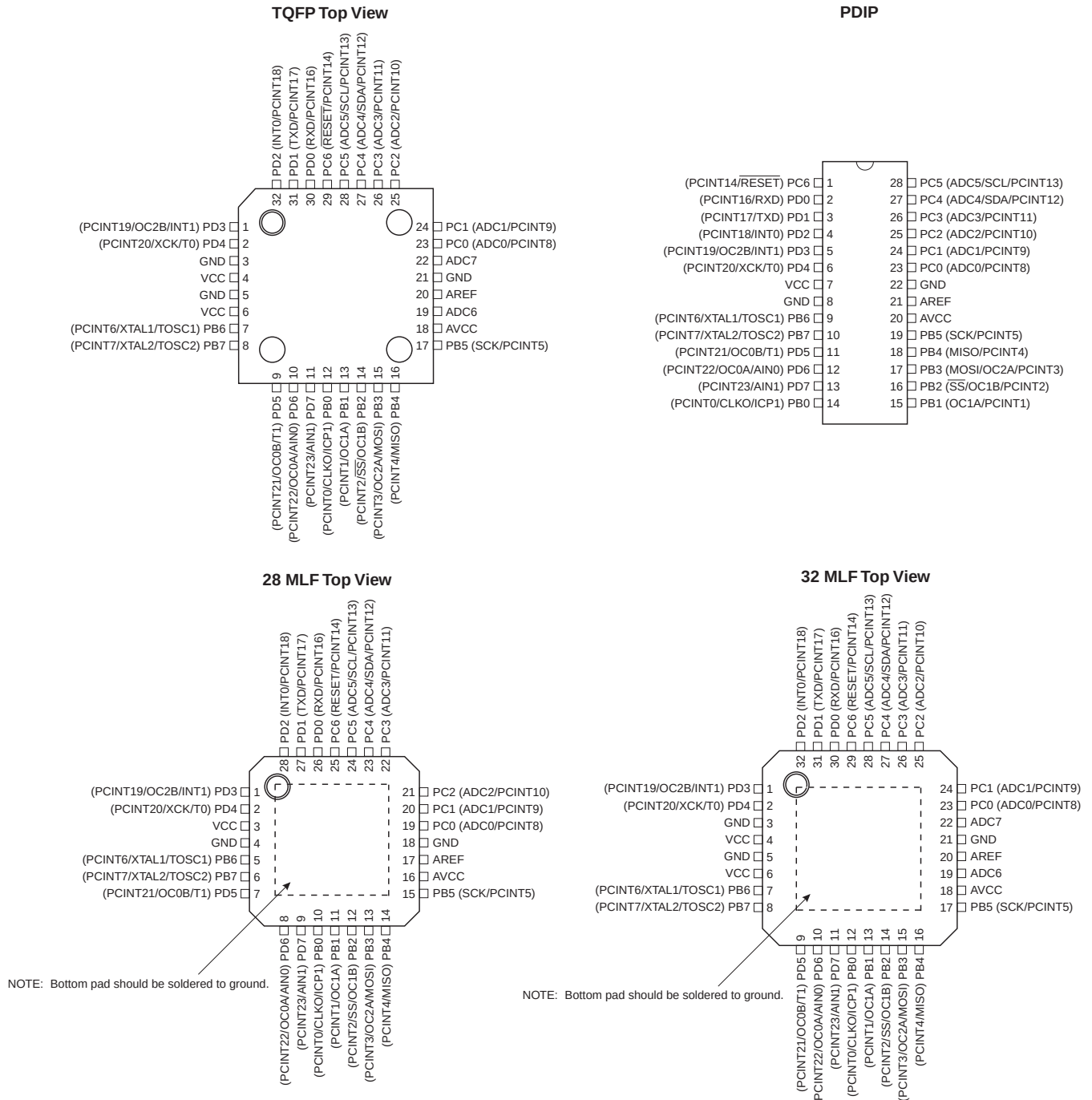
Figure 1-1. Pinout ATmega48/88/1682545L
